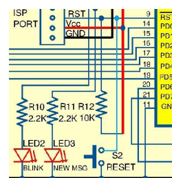
Fig. 1: Reset button S2 connected to RST pin
